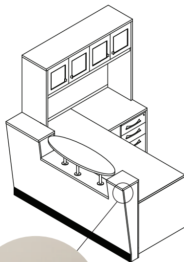
Layout REC2-2 (5474)
