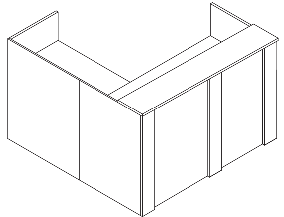
Layout REC7-2 (6666)
